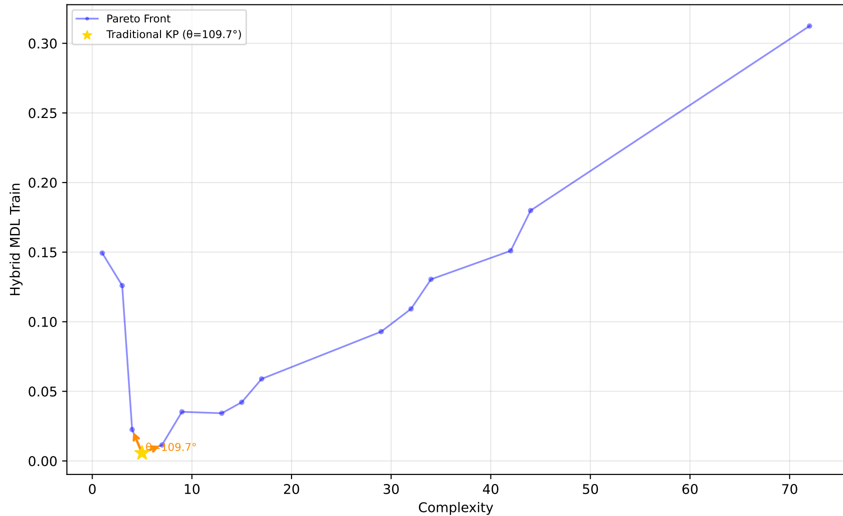
523_analcatdata_neavote - Run 30 - SVP - Hybrid MDL Train \lambda_1=0.00, \lambda_2=0.90, \lambda_3=0.00 | Difficulty: 1.00 | Method: hmr
