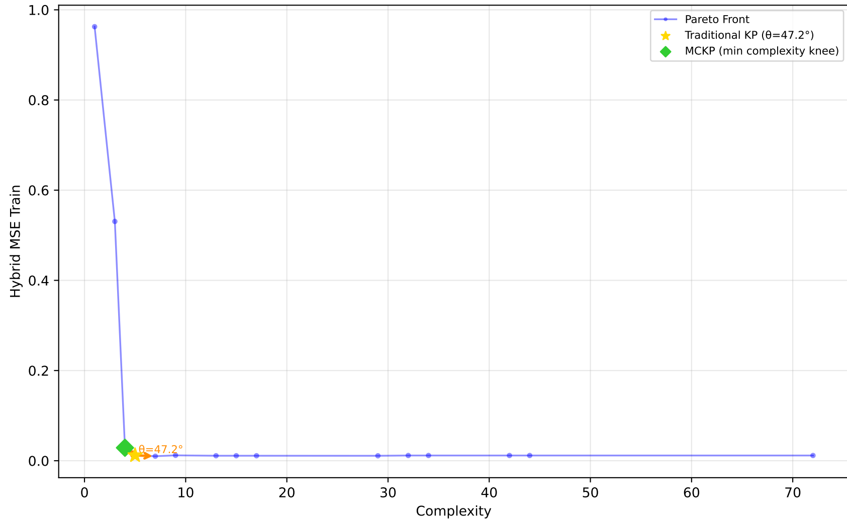
523_analcatdata_neavote - Run 30 - SVP - Hybrid MSE Train \lambda_1=0.00, \lambda_2=0.20, \lambda_3=0.00 | Difficulty: 1.00 | Method: hmr
