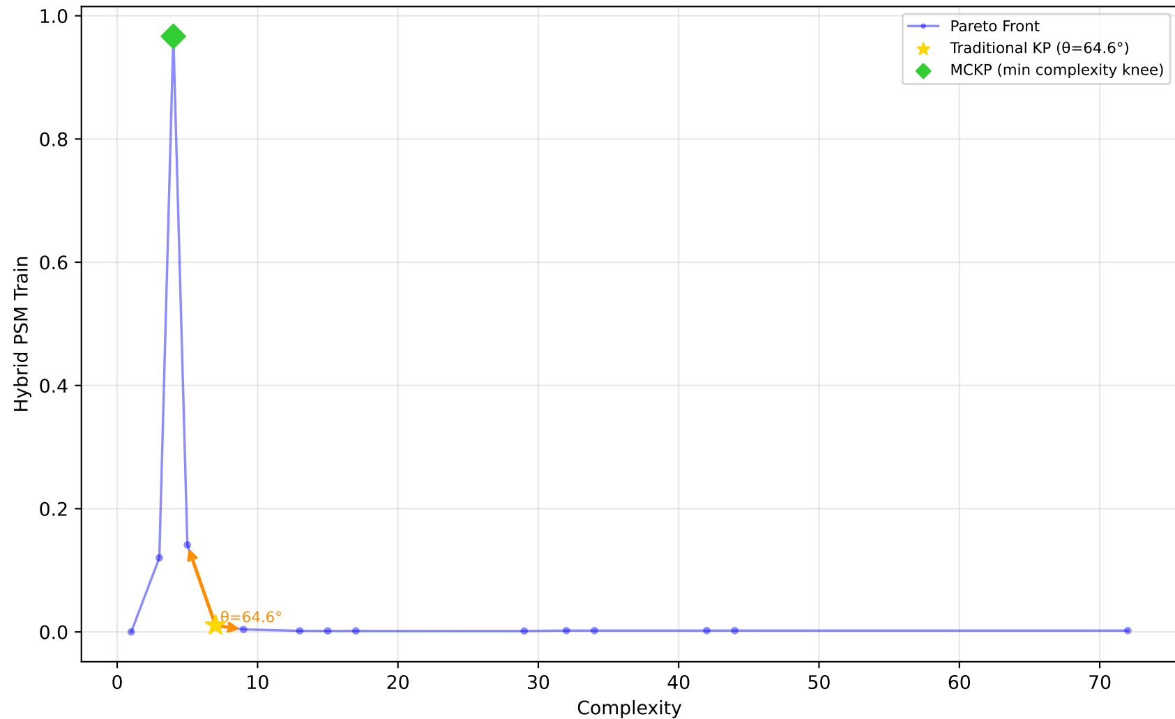
523_analcatdata_neavote - Run 30 - SVP - Hybrid PSM Train \lambda_1=0.00 , \lambda_2=0.20 , \lambda_3=0.00 | Difficulty: 1.00 | Method: hmr
