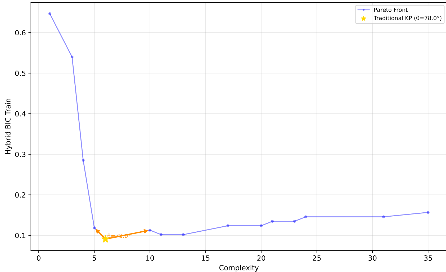
523_analcatdata_neavote - Run 3 - MVP - Hybrid BIC Train \lambda_1=0.00 , \lambda_2=0.10 , \lambda_3=0.00 | Difficulty: 1.00 | Method: hmr
