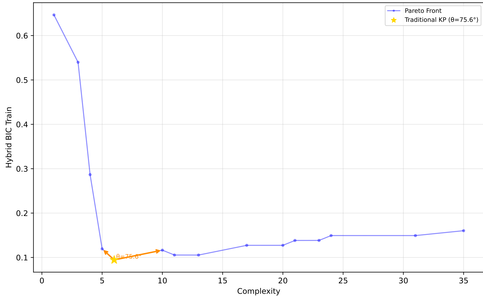
523_analcatdata_neavote - Run 3 - MVP - Hybrid BIC Train \lambda_1=0.00 , \lambda_2=0.40 , \lambda_3=0.00 | Difficulty: 1.00 | Method: hmr
