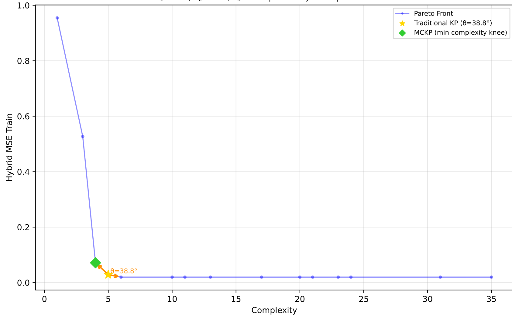
523_analcatdata_neavote - Run 3 - MVP - Hybrid MSE Train \lambda_1=0.00, \lambda_2=0.10, \lambda_3=0.00 | Difficulty: 1.00 | Method: hmr
