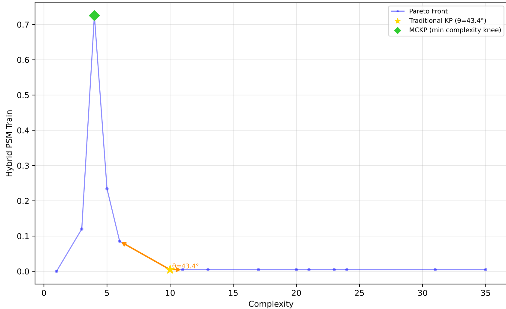
523_analcatdata_neavote - Run 3 - MVP - Hybrid PSM Train \lambda_1=0.00 , \lambda_2=0.40 , \lambda_3=0.00 | Difficulty: 1.00 | Method: hmr
