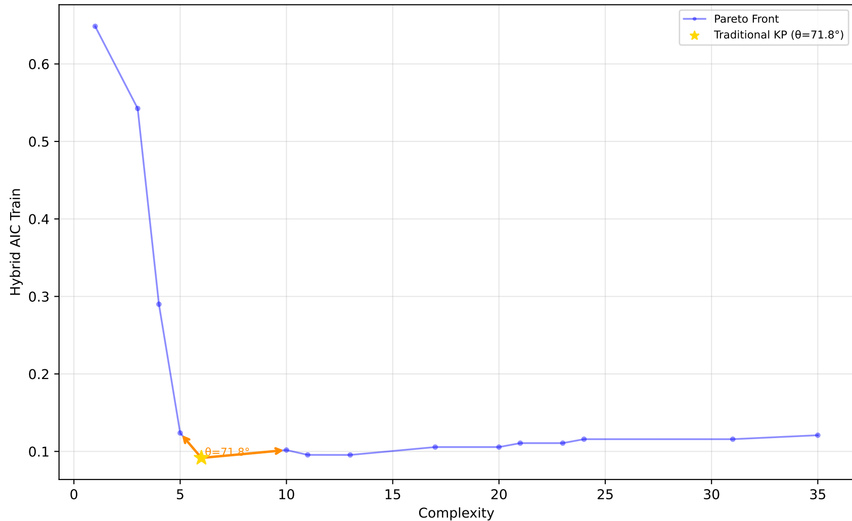
523_analcatdata_neavote - Run 3 - SVP - Hybrid AIC Train \lambda_1=0.00 , \lambda_2=0.20 , \lambda_3=0.00 | Difficulty: 1.00 | Method: hmr
