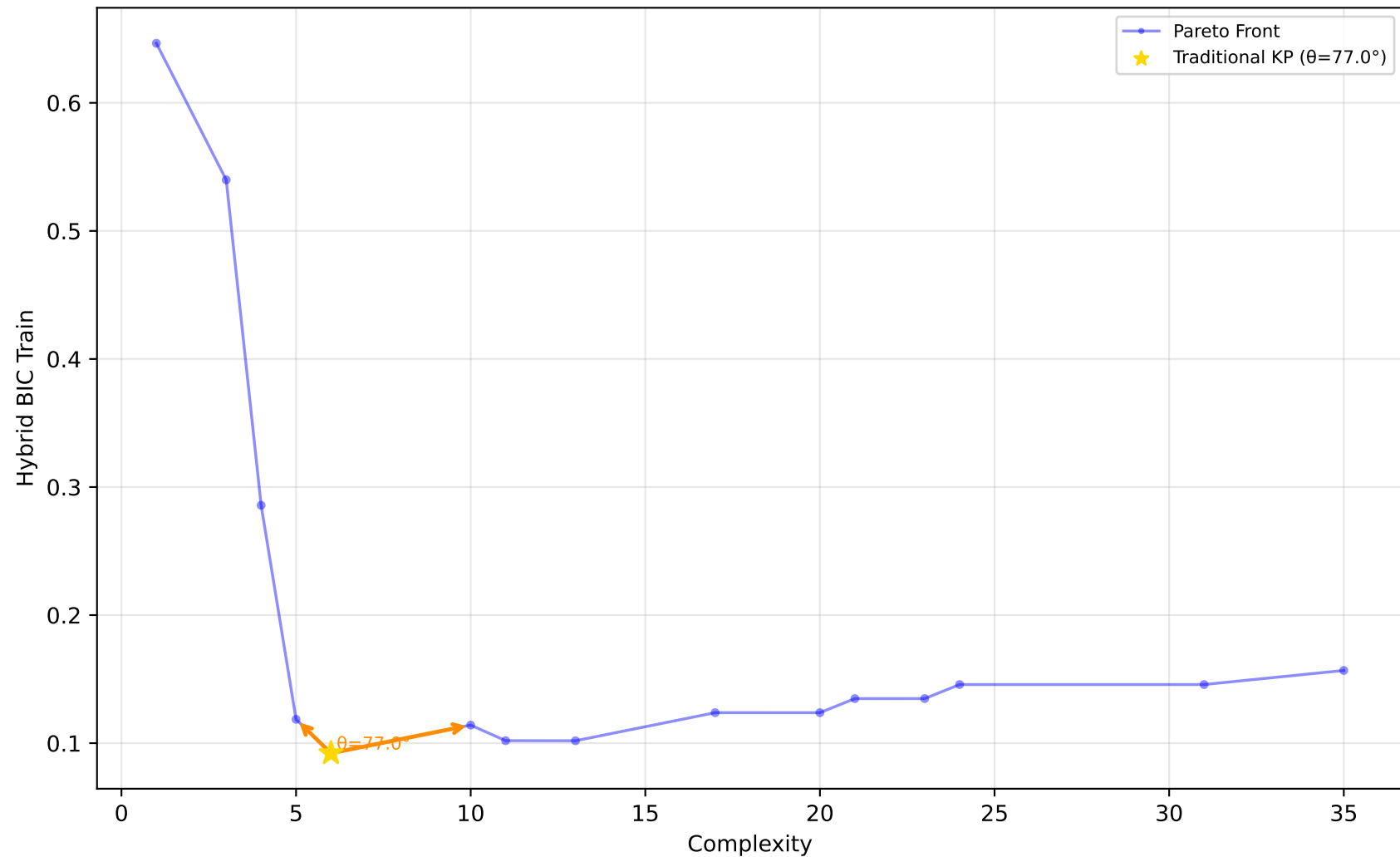
523_analcatdata_neavote - Run 3 - SVP - Hybrid BIC Train \lambda_1=0.00, \lambda_2=0.20, \lambda_3=0.00 | Difficulty: 1.00 | Method: hmr
