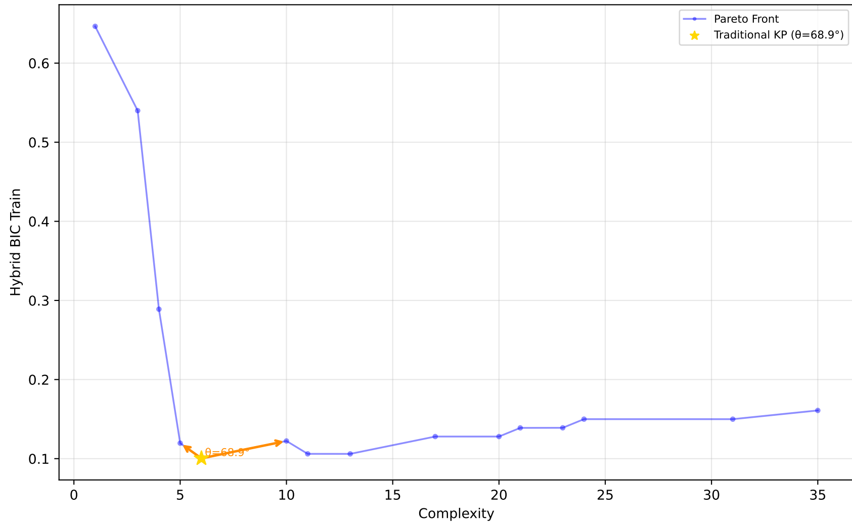
523_analcatdata_neavote - Run 3 - SVP - Hybrid BIC Train \lambda_1=0.00 , \lambda_2=0.90 , \lambda_3=0.00 | Difficulty: 1.00 | Method: hmr
