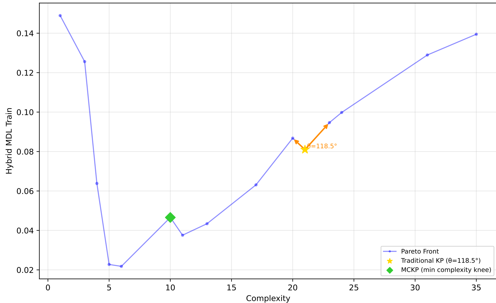
523_analcatdata_neavote - Run 3 - SVP - Hybrid MDL Train \lambda_1=0.00 , \lambda_2=0.20 , \lambda_3=0.00 | Difficulty: 1.00 | Method: hmr
