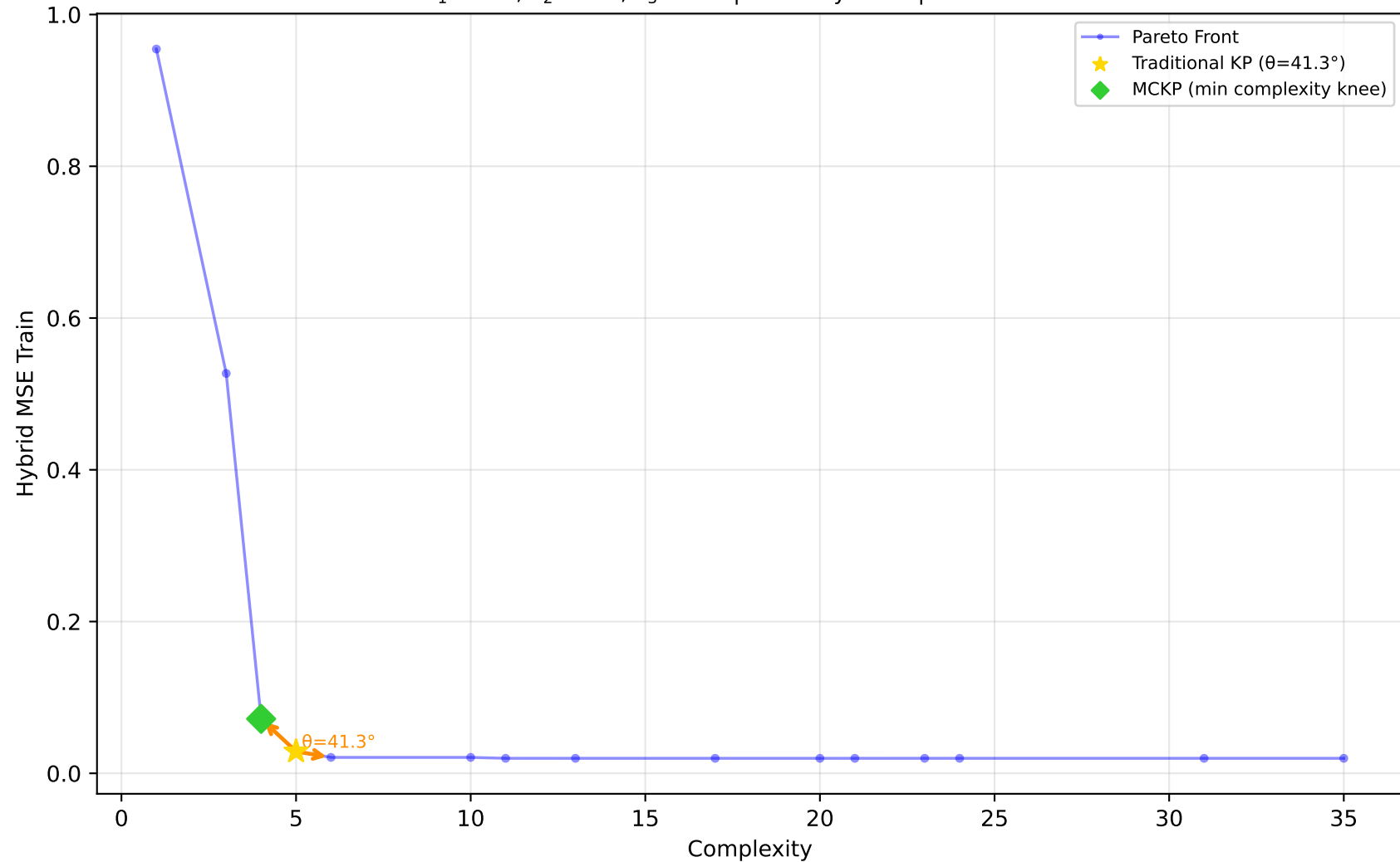
523_analcatdata_neavote - Run 3 - SVP - Hybrid MSE Train \lambda_1=0.00 , \lambda_2=0.20 , \lambda_3=0.00 | Difficulty: 1.00 | Method: hmr
