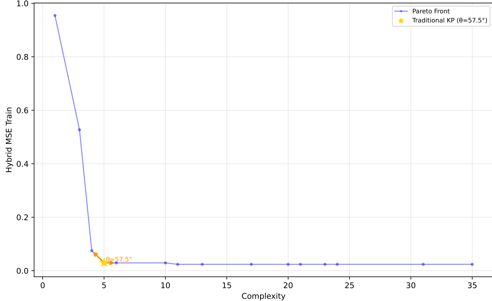
523_analcatdata_neavote - Run 3 - SVP - Hybrid MSE Train \lambda_1=0.00, \lambda_2=0.90, \lambda_3=0.00 | Difficulty: 1.00 | Method: hmr
