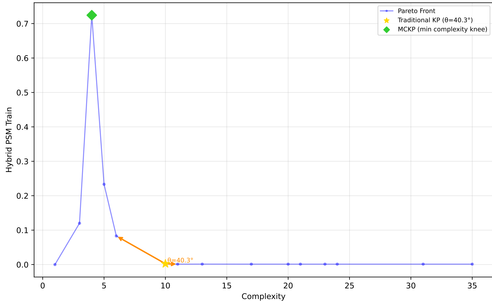
523_analcatdata_neavote - Run 3 - SVP - Hybrid PSM Train \lambda_1=0.00 , \lambda_2=0.20 , \lambda_3=0.00 | Difficulty: 1.00 | Method: hmr
