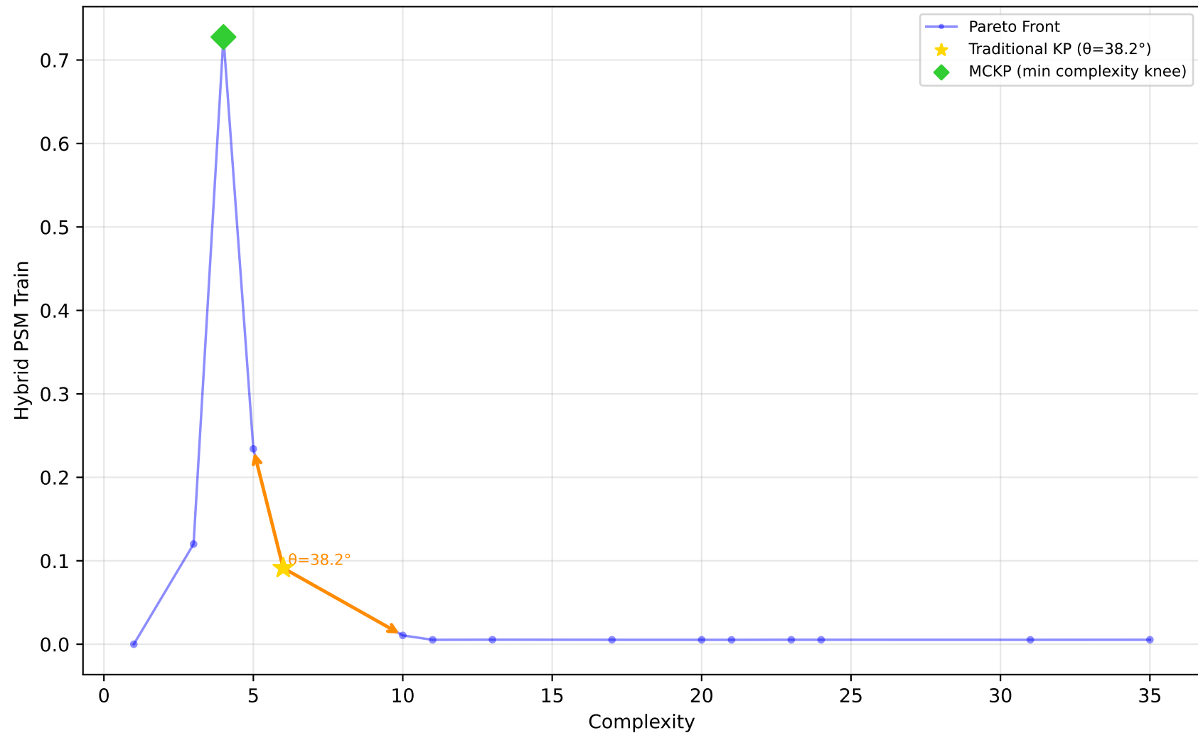
523_analcatdata_neavote - Run 3 - SVP - Hybrid PSM Train \lambda_1=0.00 , \lambda_2=0.90 , \lambda_3=0.00 | Difficulty: 1.00 | Method: hmr
