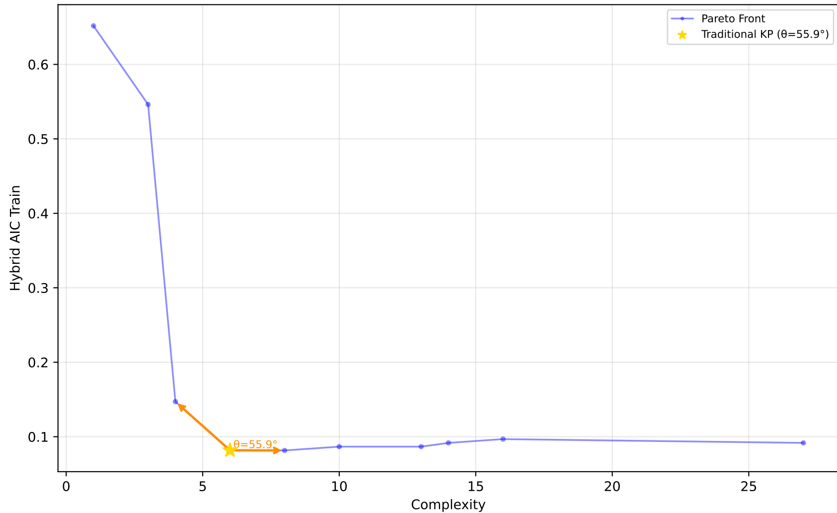
523_analcatdata_neavote - Run 4 - MVP - Hybrid AIC Train \lambda_1=0.00 , \lambda_2=0.10 , \lambda_3=0.00 | Difficulty: 1.00 | Method: hmr
