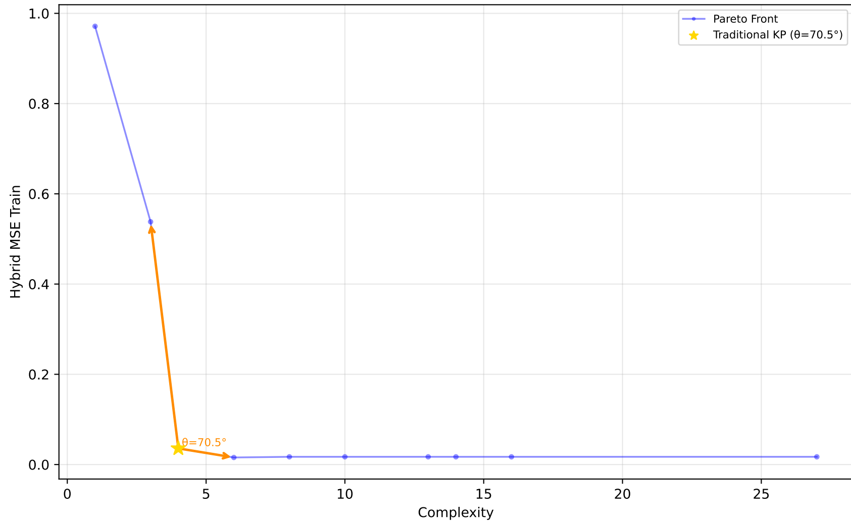
523_analcatdata_neavote - Run 4 - MVP - Hybrid MSE Train \lambda_1=0.00, \lambda_2=0.10, \lambda_3=0.00 | Difficulty: 1.00 | Method: hmr
