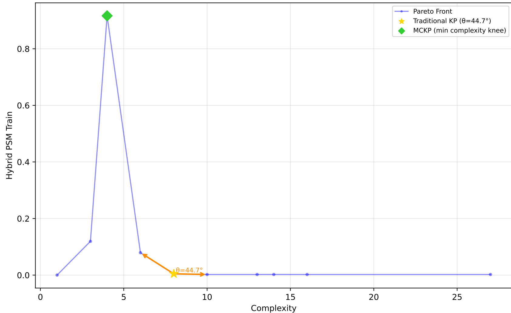
523_analcatdata_neavote - Run 4 - MVP - Hybrid PSM Train \lambda_1=0.00, \lambda_2=0.10, \lambda_3=0.00 | Difficulty: 1.00 | Method: hmr
