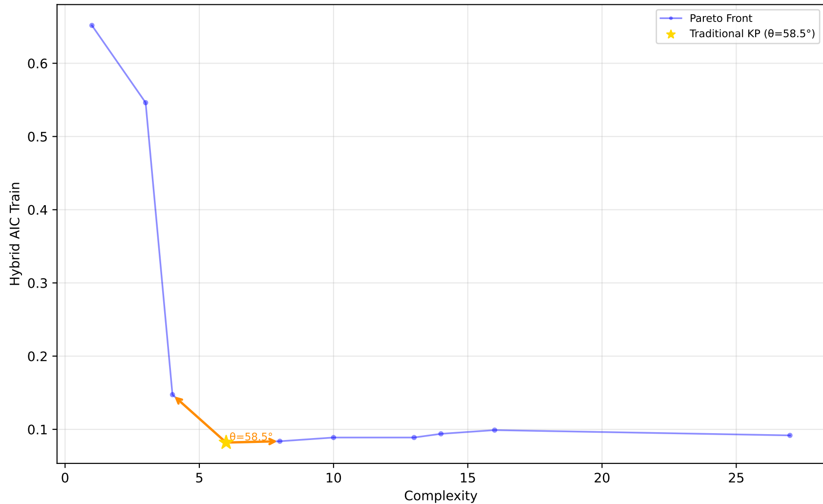
523_analcatdata_neavote - Run 4 - SVP - Hybrid AIC Train \lambda_1=0.00 , \lambda_2=0.20 , \lambda_3=0.00 | Difficulty: 1.00 | Method: hmr
