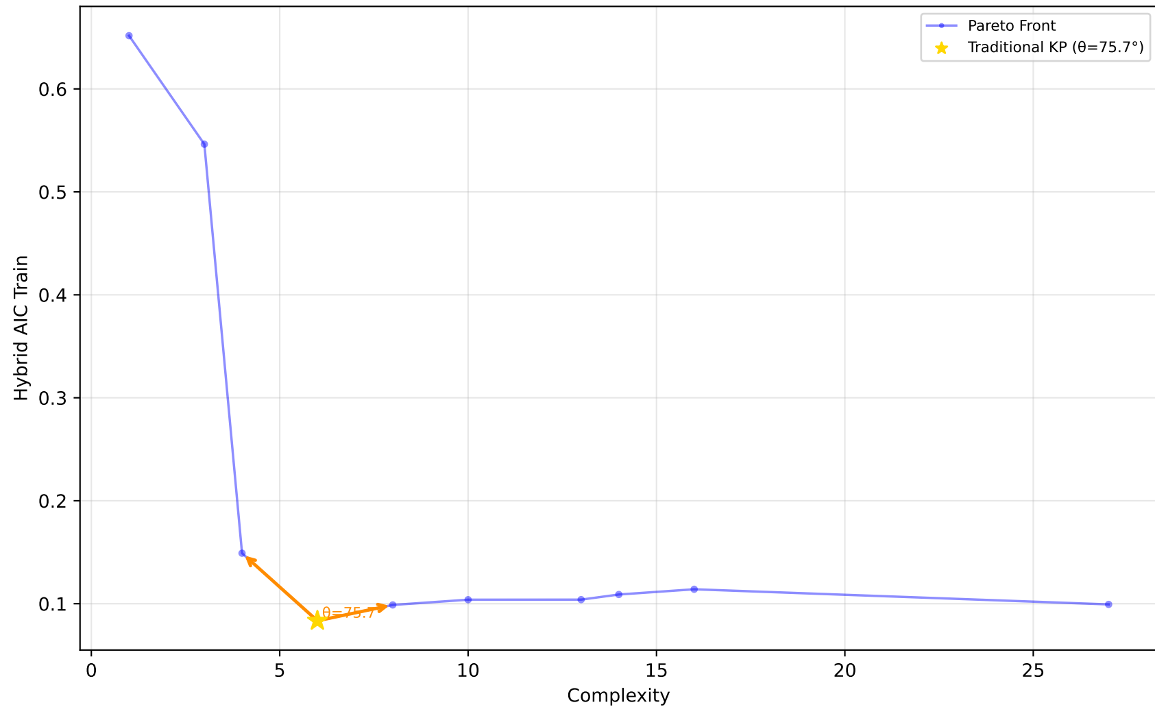
523_analcatdata_neavote - Run 4 - SVP - Hybrid AIC Train \lambda_1=0.00 , \lambda_2=0.90 , \lambda_3=0.00 | Difficulty: 1.00 | Method: hmr
