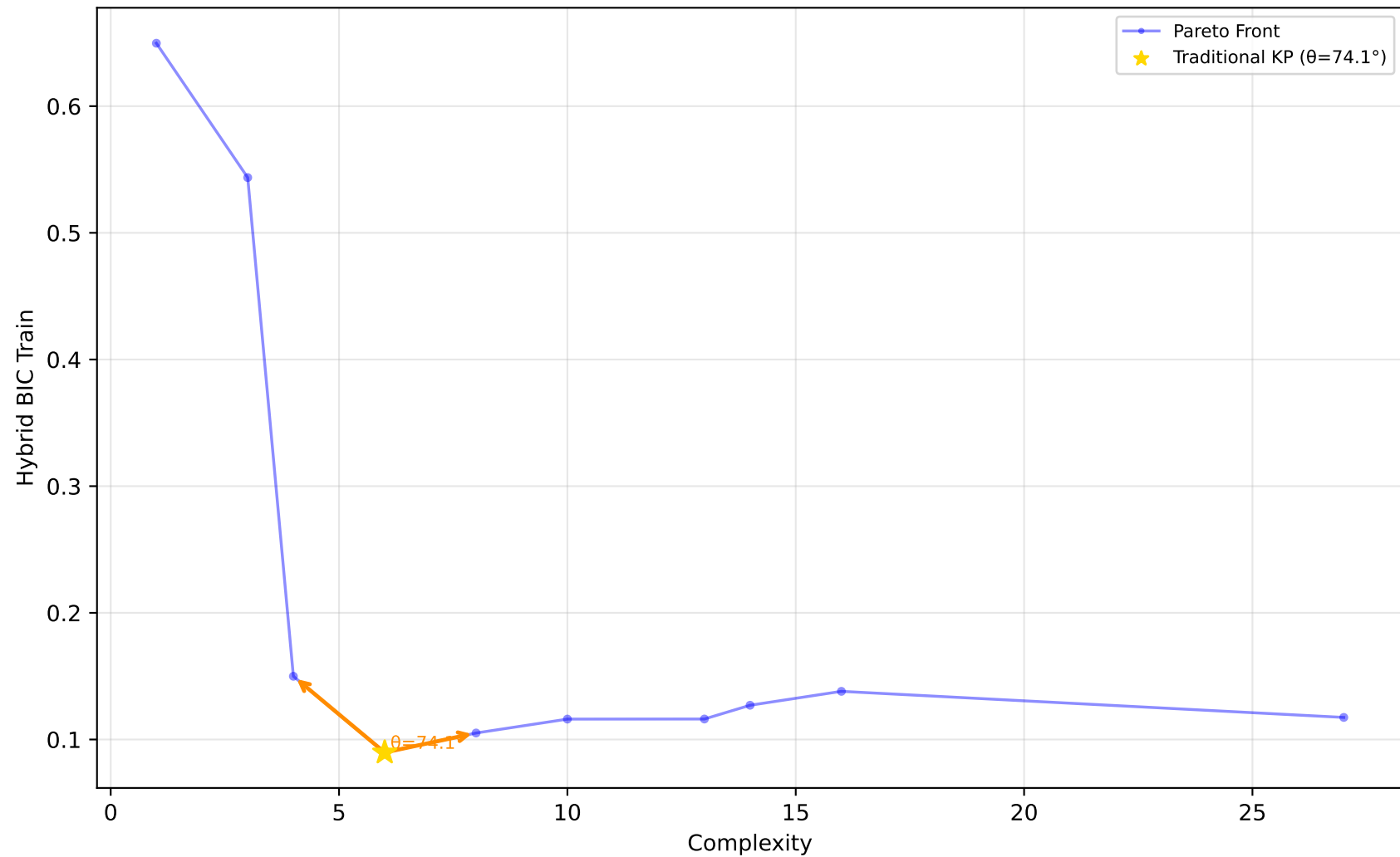
523_analcatdata_neavote - Run 4 - SVP - Hybrid BIC Train \lambda_1=0.00, \lambda_2=0.90, \lambda_3=0.00 | Difficulty: 1.00 | Method: hmr
