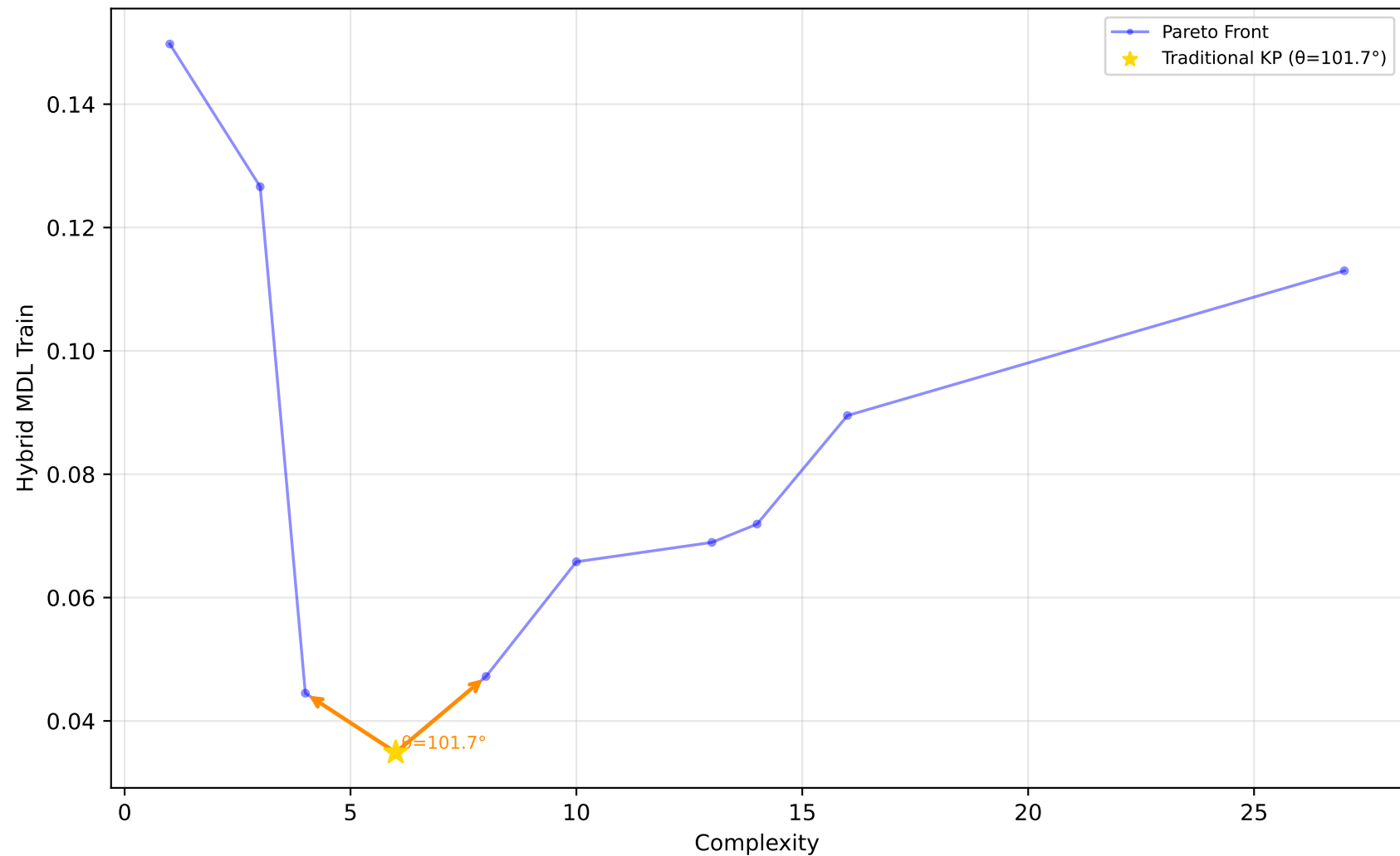
523_analcatdata_neavote - Run 4 - SVP - Hybrid MDL Train \lambda_1=0.00, \lambda_2=0.90, \lambda_3=0.00 | Difficulty: 1.00 | Method: hmr
