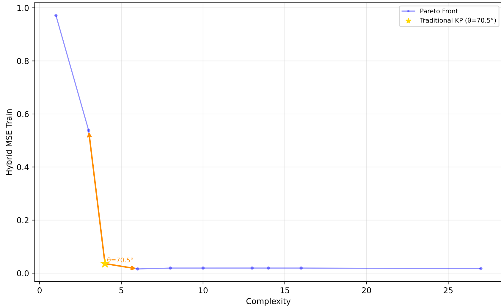
523_analcatdata_neavote - Run 4 - SVP - Hybrid MSE Train \lambda_1=0.00, \lambda_2=0.20, \lambda_3=0.00 | Difficulty: 1.00 | Method: hmr
