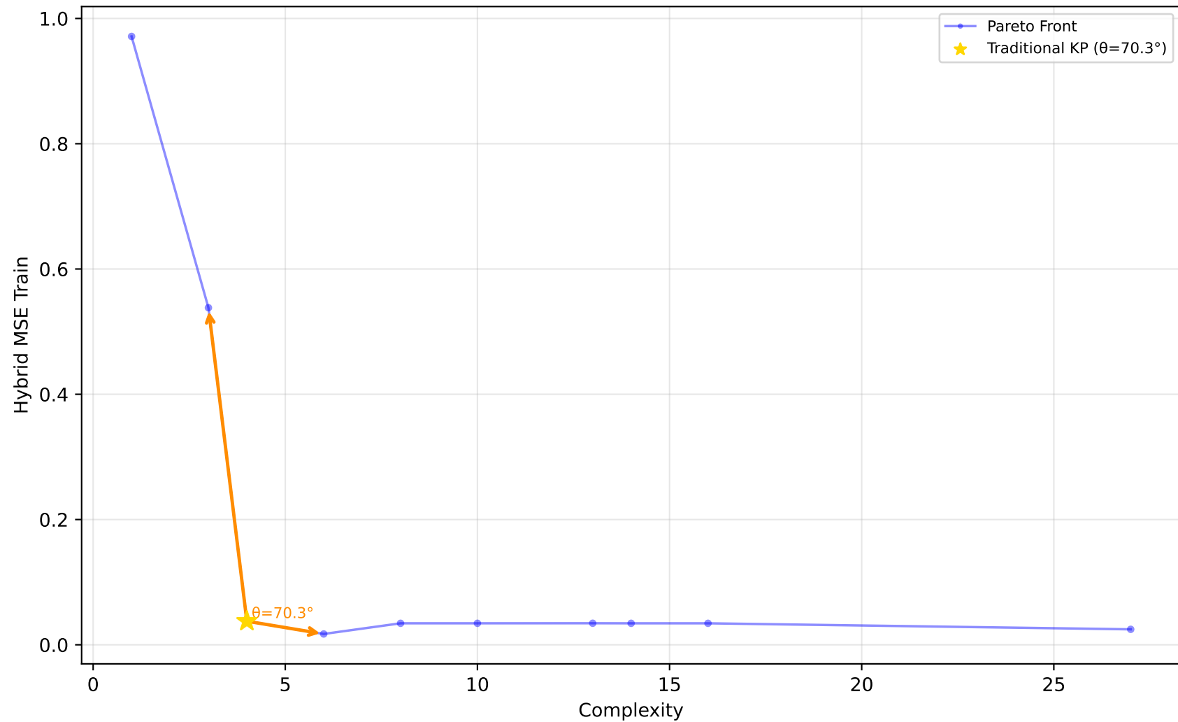
523_analcatdata_neavote - Run 4 - SVP - Hybrid MSE Train \lambda_1=0.00, \lambda_2=0.90, \lambda_3=0.00 | Difficulty: 1.00 | Method: hmr
