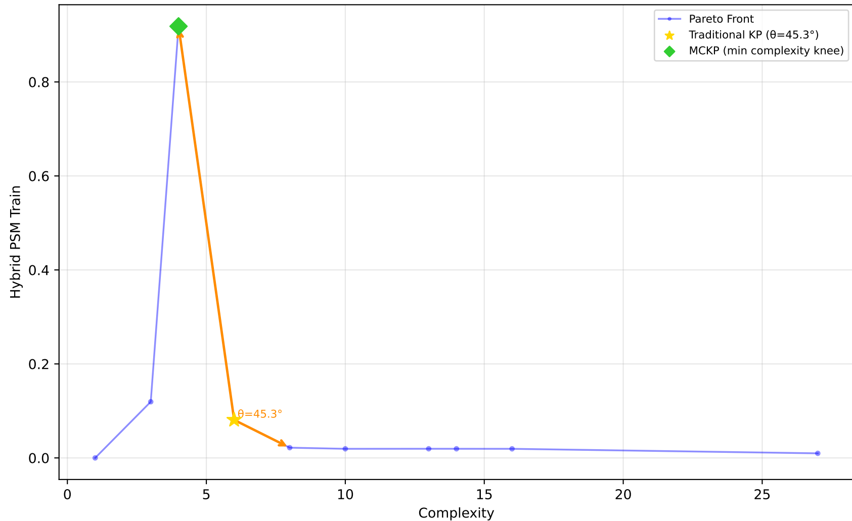
523_analcatdata_neavote - Run 4 - SVP - Hybrid PSM Train \lambda_1=0.00, \lambda_2=0.90, \lambda_3=0.00 | Difficulty: 1.00 | Method: hmr
