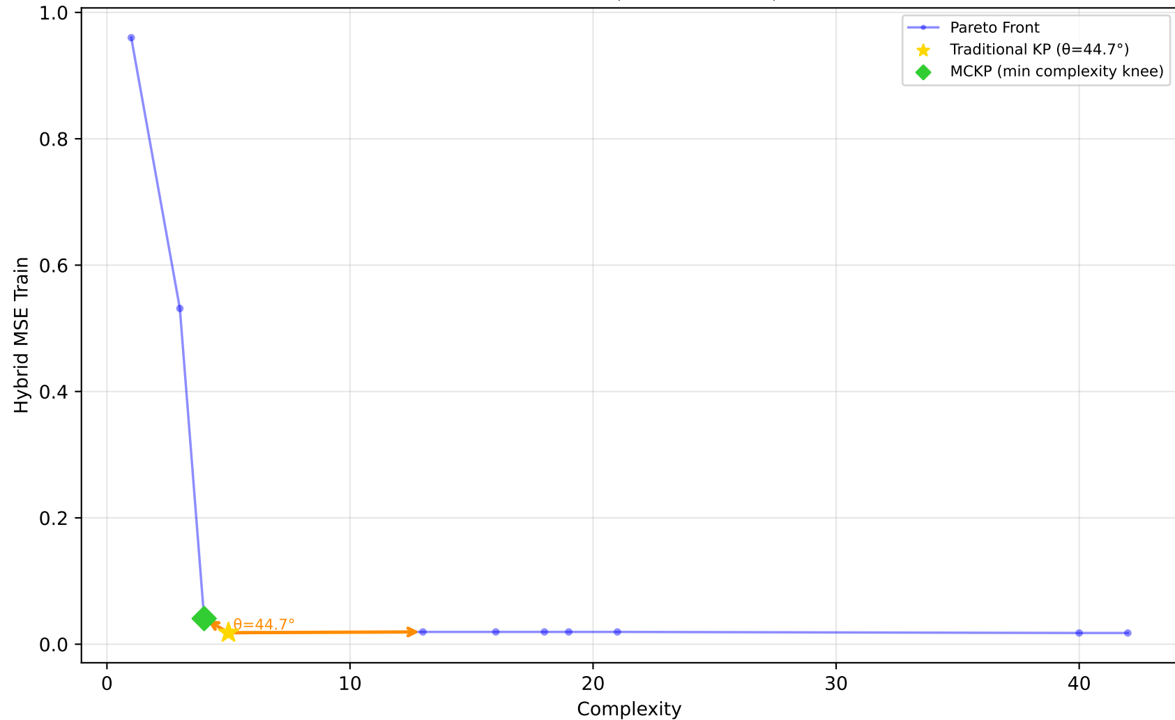
523_analcatdata_neavote - Run 5 - MVP - Hybrid MSE Train \lambda_1=0.00, \lambda_2=0.40, \lambda_3=0.00 | Difficulty: 1.00 | Method: hmr
