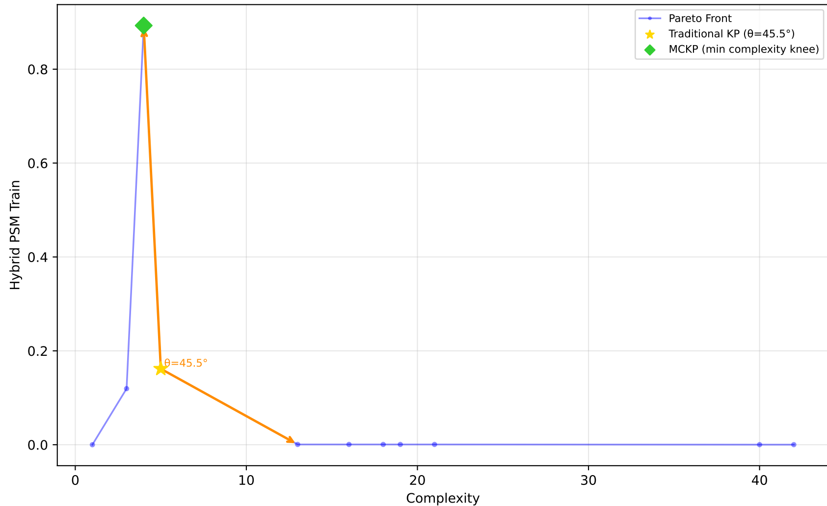
523_analcatdata_neavote - Run 5 - MVP - Hybrid PSM Train \lambda_1=0.00 , \lambda_2=0.10 , \lambda_3=0.00 | Difficulty: 1.00 | Method: hmr
