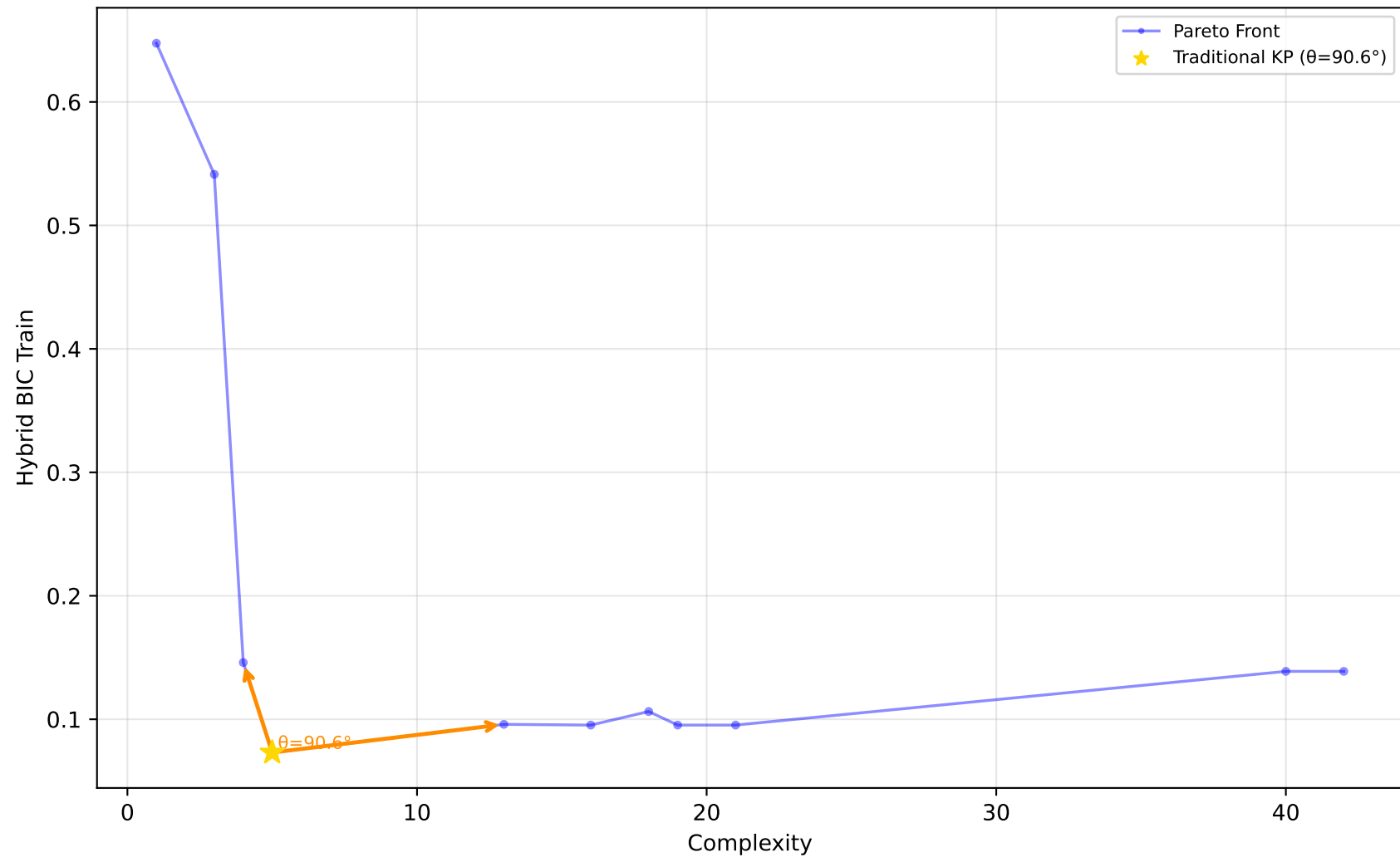
523_analcatdata_neavote - Run 5 - SVP - Hybrid BIC Train \lambda_1=0.00, \lambda_2=0.20, \lambda_3=0.00 | Difficulty: 1.00 | Method: hmr
