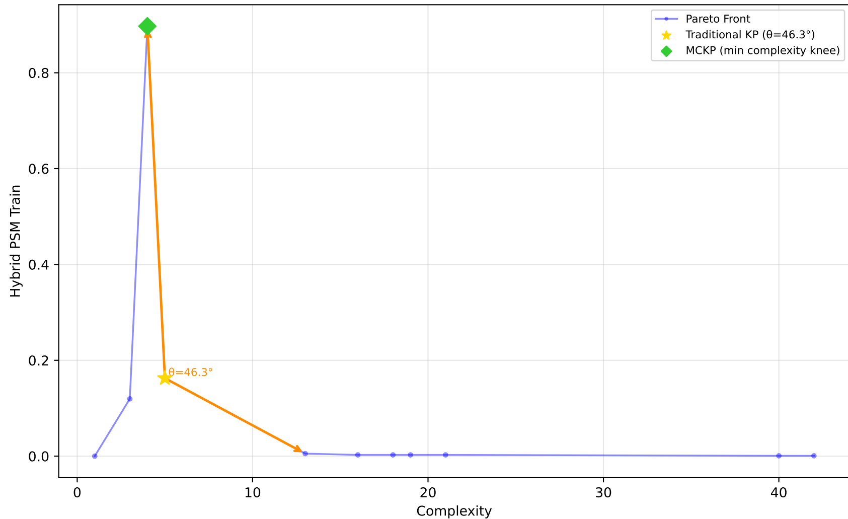
523_analcatdata_neavote - Run 5 - SVP - Hybrid PSM Train \lambda_1=0.00 , \lambda_2=0.90 , \lambda_3=0.00 | Difficulty: 1.00 | Method: hmr
