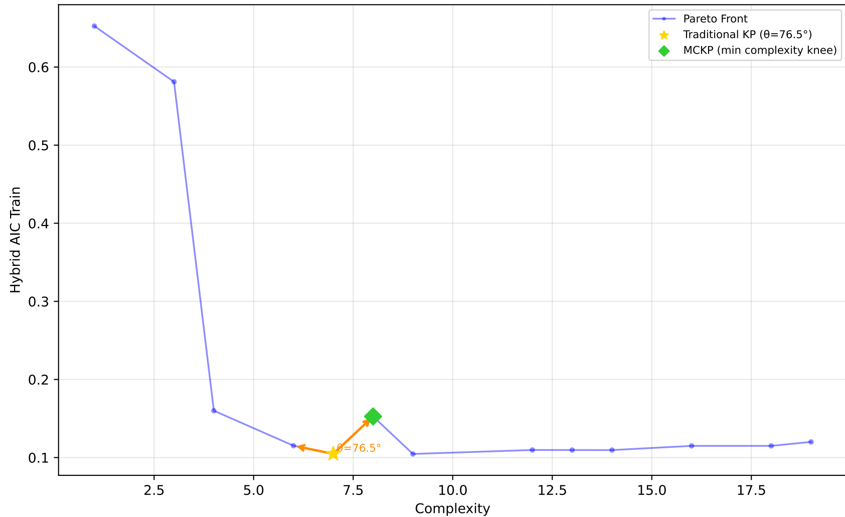
523_analcatdata_neavote - Run 6 - MVP - Hybrid AIC Train \lambda_1=0.00 , \lambda_2=0.10 , \lambda_3=0.00 | Difficulty: 1.00 | Method: hmr
