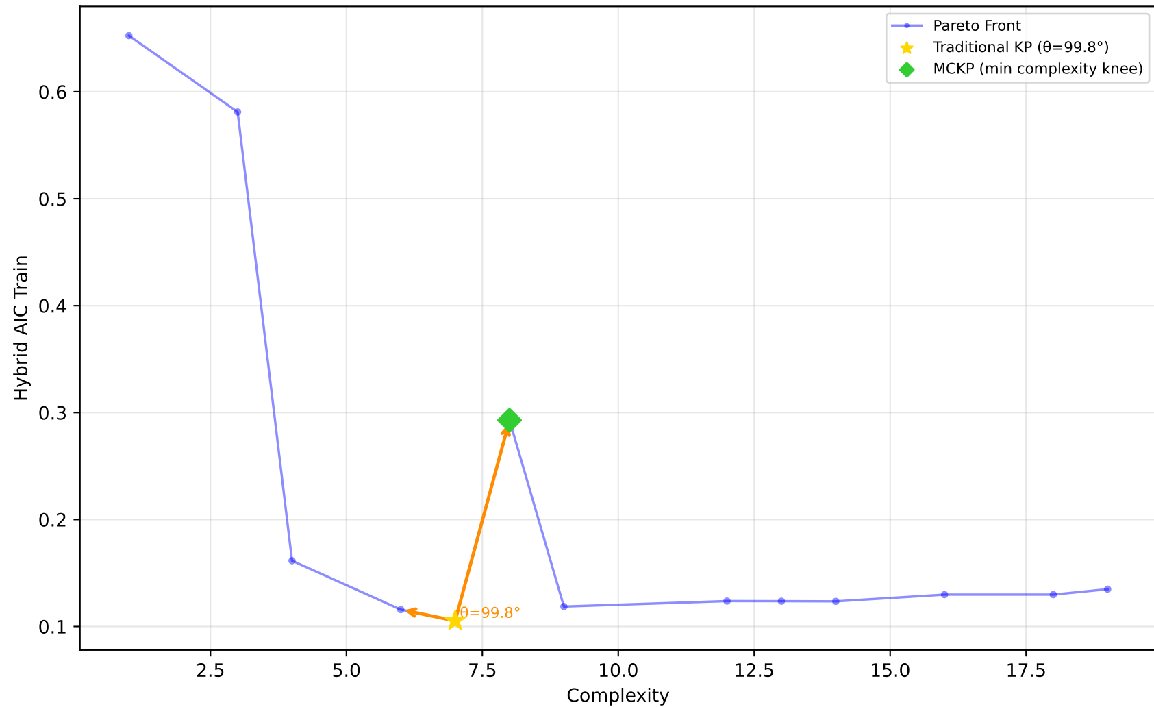
523_analcatdata_neavote - Run 6 - MVP - Hybrid AIC Train \lambda_1=0.00 , \lambda_2=0.40 , \lambda_3=0.00 | Difficulty: 1.00 | Method: hmr
