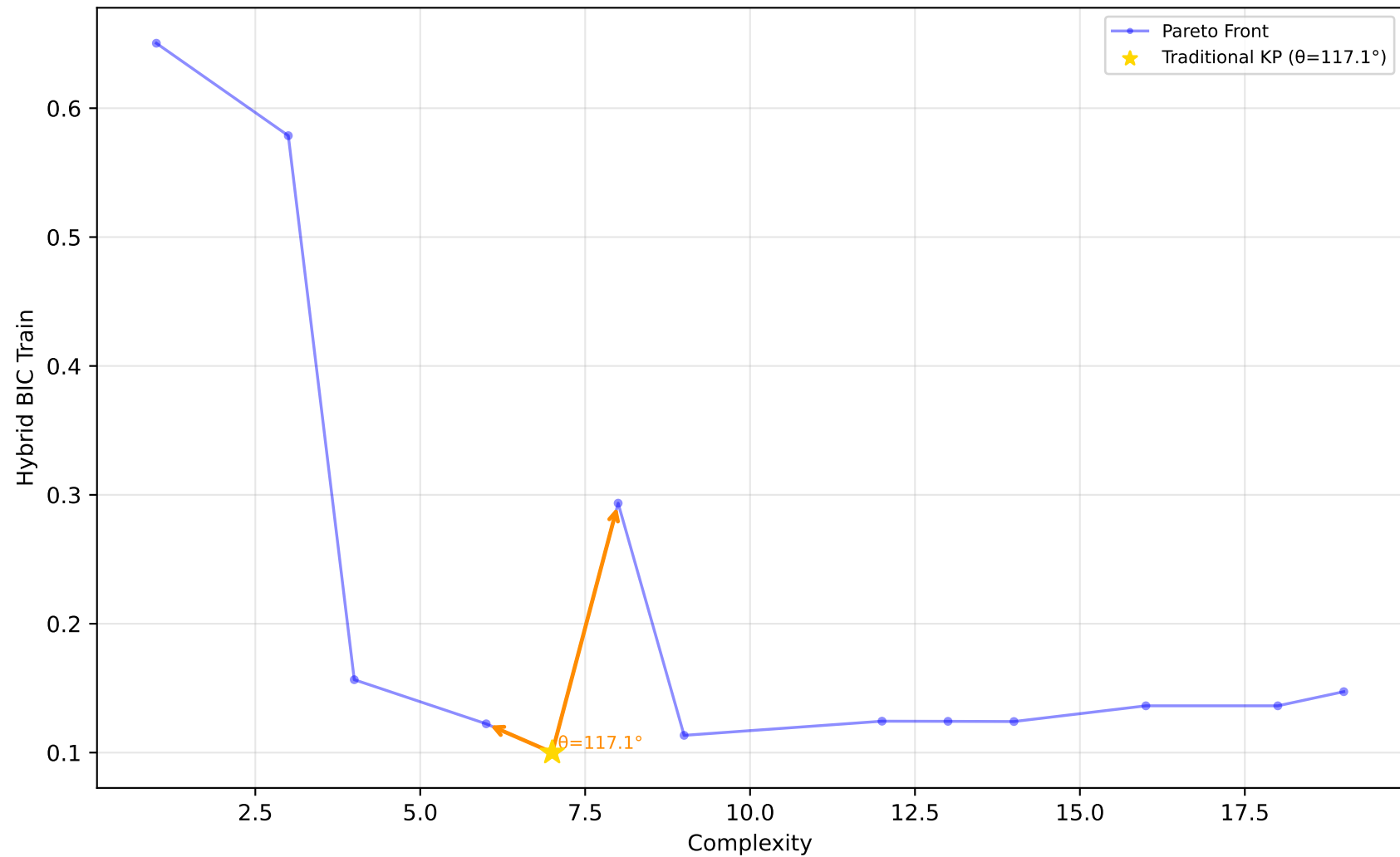
523_analcatdata_neavote - Run 6 - MVP - Hybrid BIC Train \lambda_1=0.00 , \lambda_2=0.40 , \lambda_3=0.00 | Difficulty: 1.00 | Method: hmr
