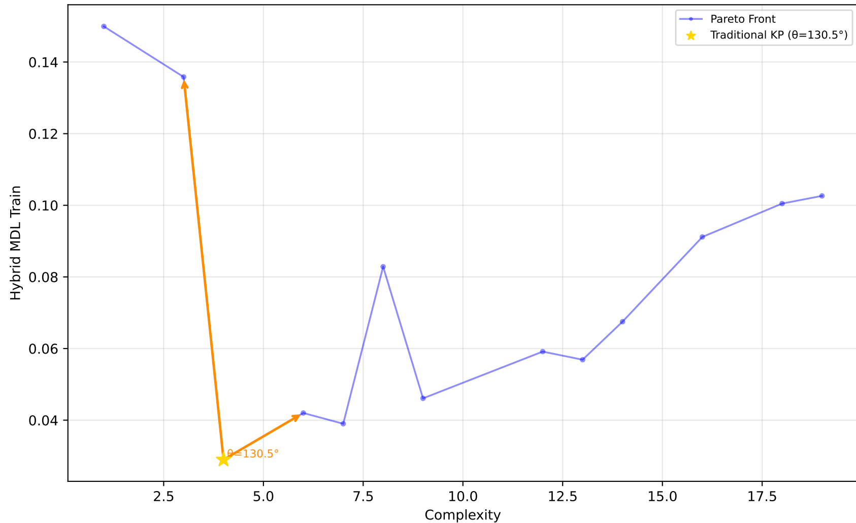
523_analcatdata_neavote - Run 6 - MVP - Hybrid MDL Train \lambda_1=0.00 , \lambda_2=0.10 , \lambda_3=0.00 | Difficulty: 1.00 | Method: hmr
