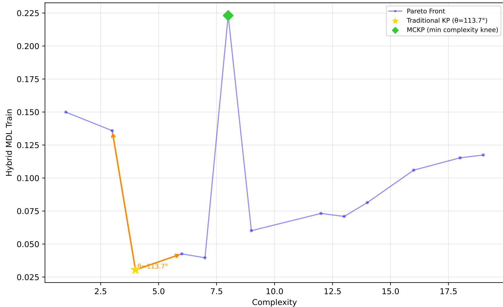
523_analcatdata_neavote - Run 6 - MVP - Hybrid MDL Train \lambda_1=0.00 , \lambda_2=0.40 , \lambda_3=0.00 | Difficulty: 1.00 | Method: hmr
