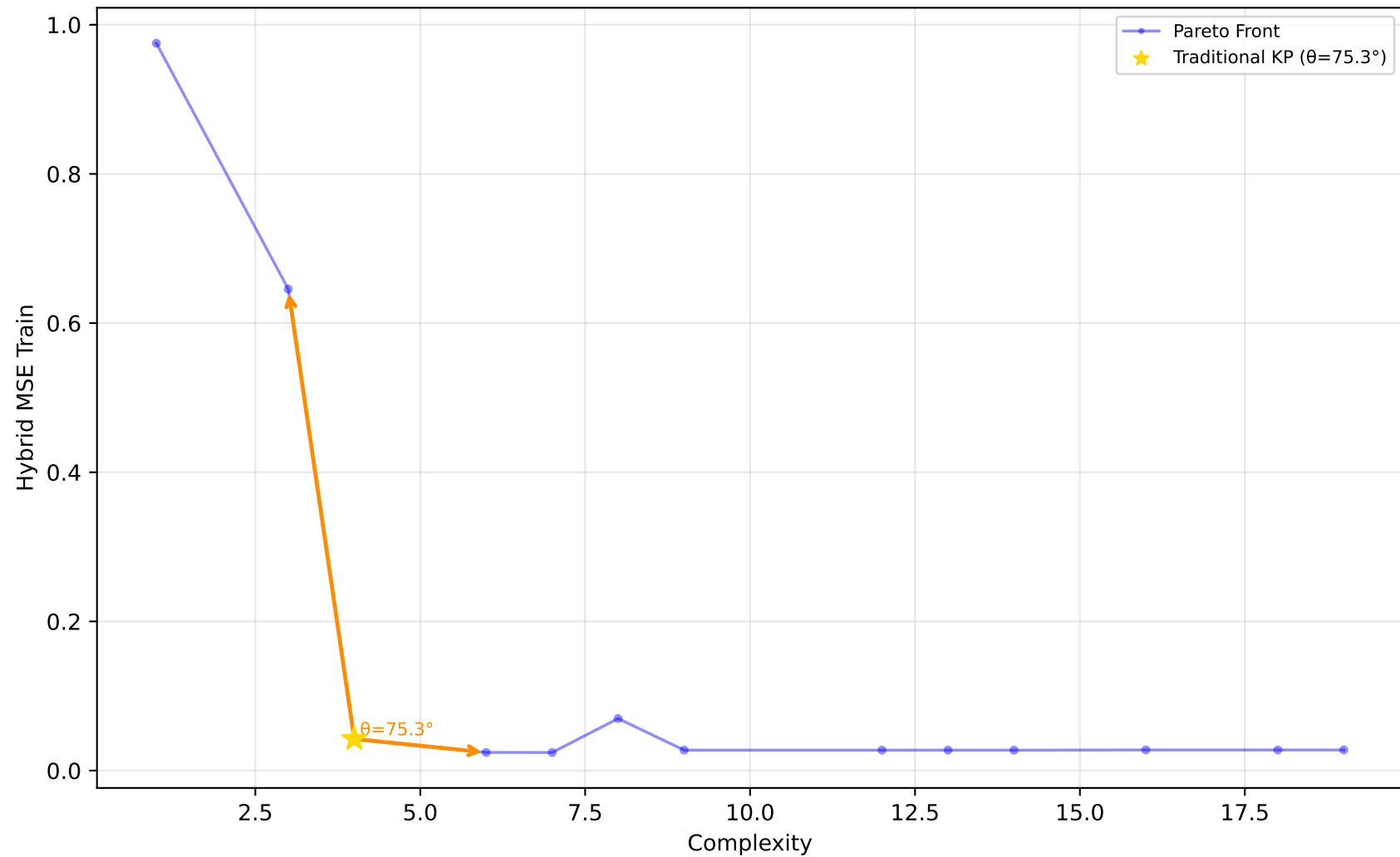
523_analcatdata_neavote - Run 6 - MVP - Hybrid MSE Train \lambda_1=0.00, \lambda_2=0.10, \lambda_3=0.00 | Difficulty: 1.00 | Method: hmr
