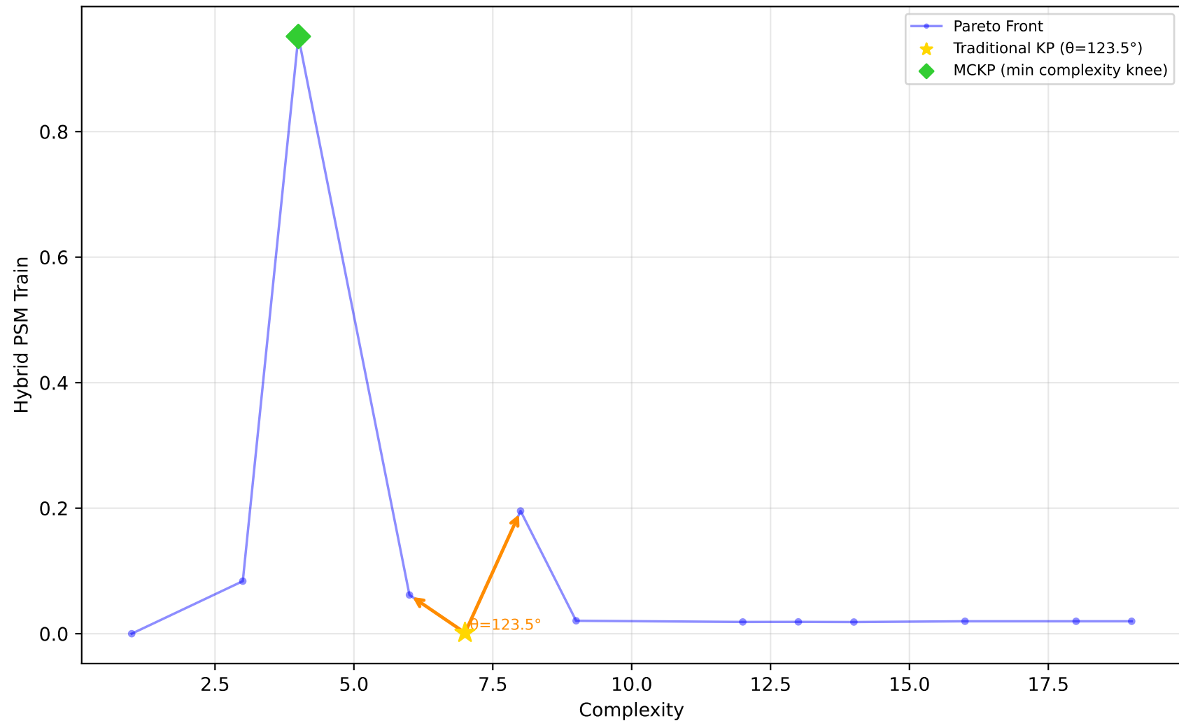
523_analcatdata_neavote - Run 6 - MVP - Hybrid PSM Train \lambda_1=0.00 , \lambda_2=0.40 , \lambda_3=0.00 | Difficulty: 1.00 | Method: hmr
