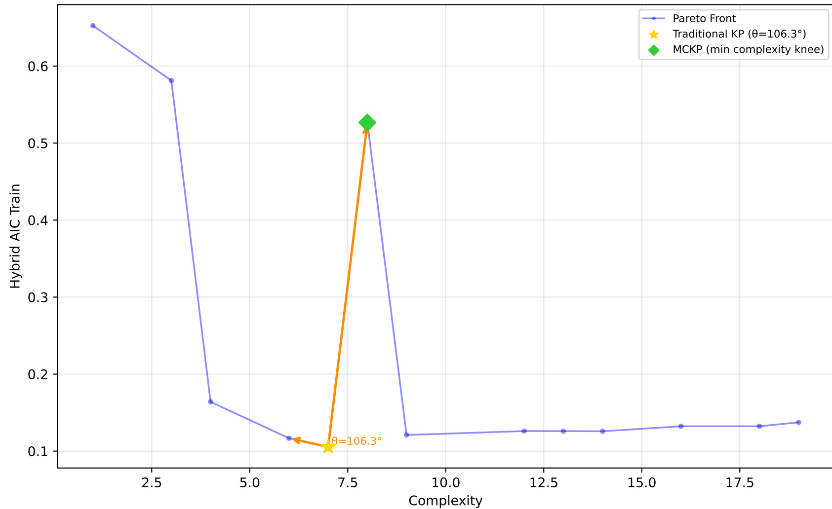
523_analcatdata_neavote - Run 6 - SVP - Hybrid AIC Train \lambda_1=0.00, \lambda_2=0.90, \lambda_3=0.00 | Difficulty: 1.00 | Method: hmr
