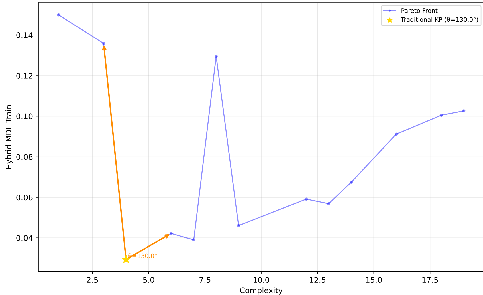
523_analcatdata_neavote - Run 6 - SVP - Hybrid MDL Train \lambda_1=0.00 , \lambda_2=0.20 , \lambda_3=0.00 | Difficulty: 1.00 | Method: hmr
