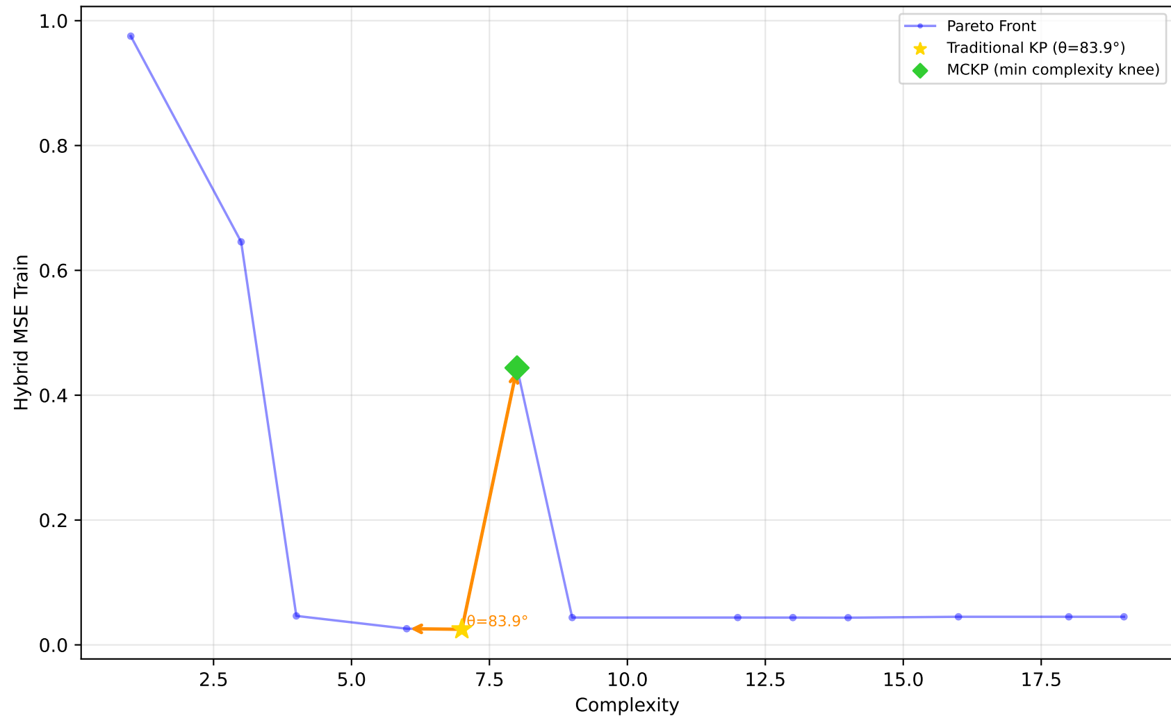
523_analcatdata_neavote - Run 6 - SVP - Hybrid MSE Train \lambda_1=0.00, \lambda_2=0.90, \lambda_3=0.00 | Difficulty: 1.00 | Method: hmr
