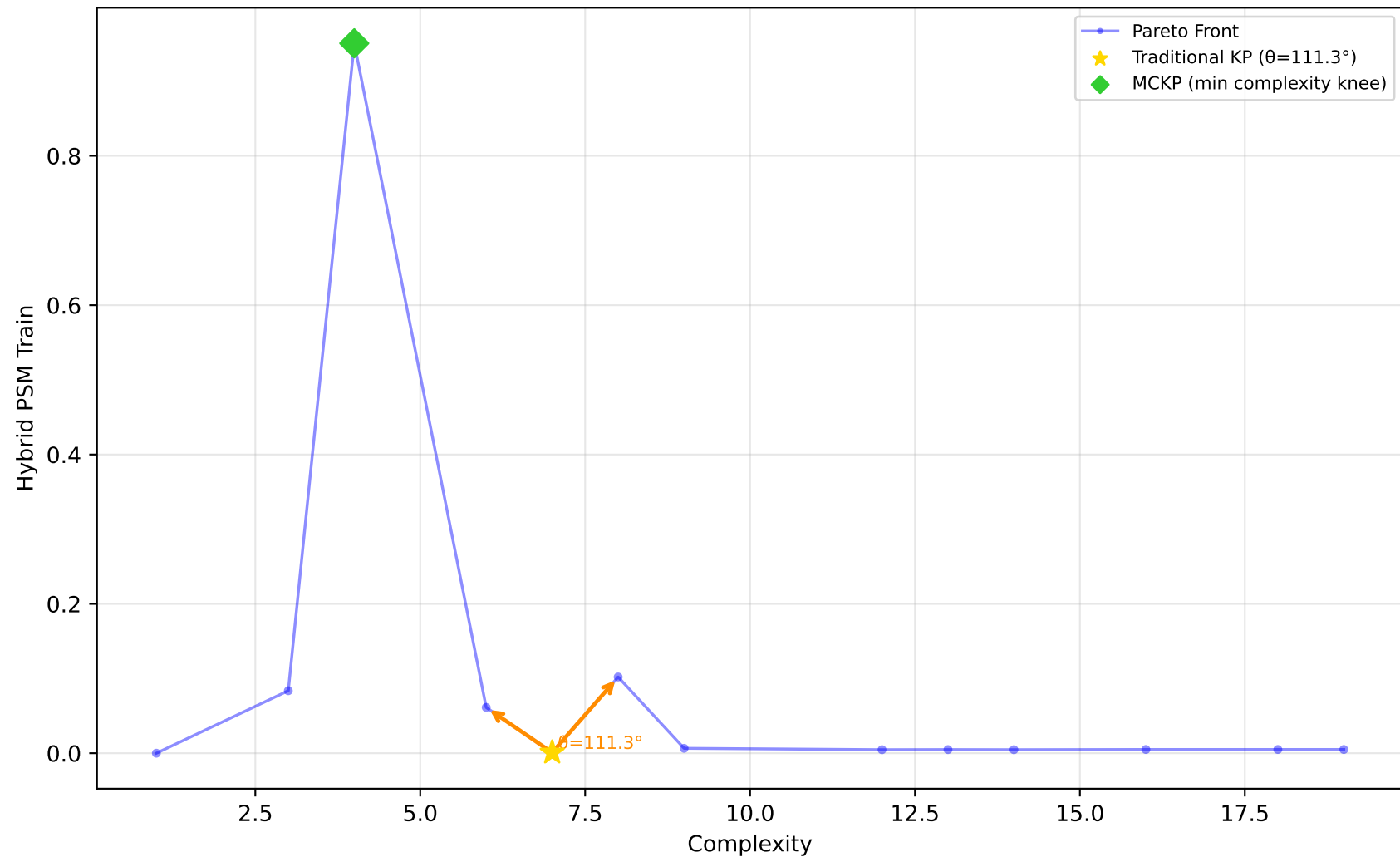
523_analcatdata_neavote - Run 6 - SVP - Hybrid PSM Train \lambda_1=0.00 , \lambda_2=0.20 , \lambda_3=0.00 | Difficulty: 1.00 | Method: hmr
