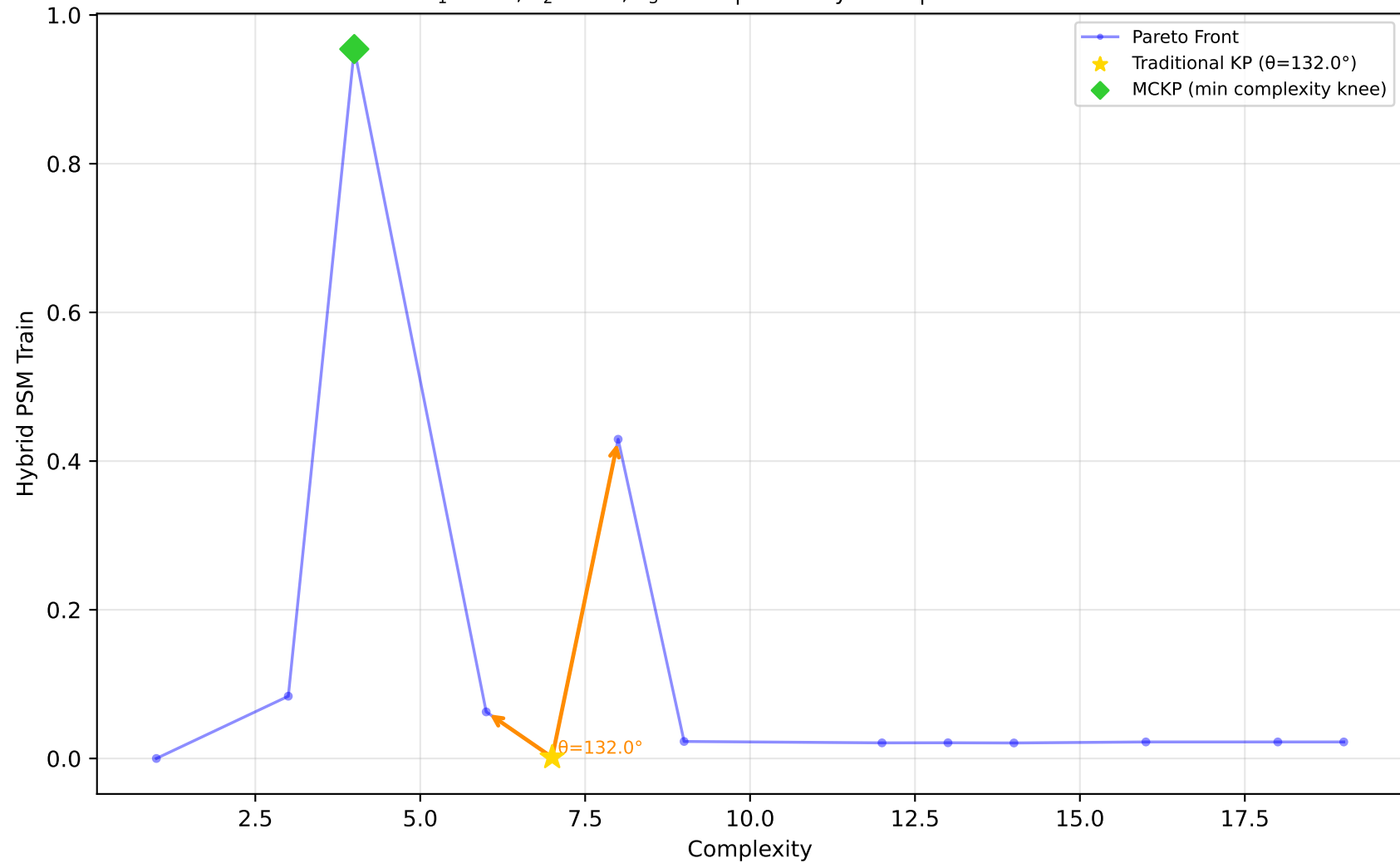
523_analcatdata_neavote - Run 6 - SVP - Hybrid PSM Train \lambda_1=0.00, \lambda_2=0.90, \lambda_3=0.00 | Difficulty: 1.00 | Method: hmr
