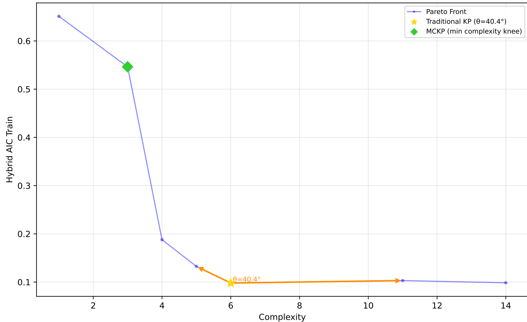
523_analcatdata_neavote - Run 7 - MVP - Hybrid AIC Train \lambda_1=0.00 , \lambda_2=0.10 , \lambda_3=0.00 | Difficulty: 1.00 | Method: hmr
