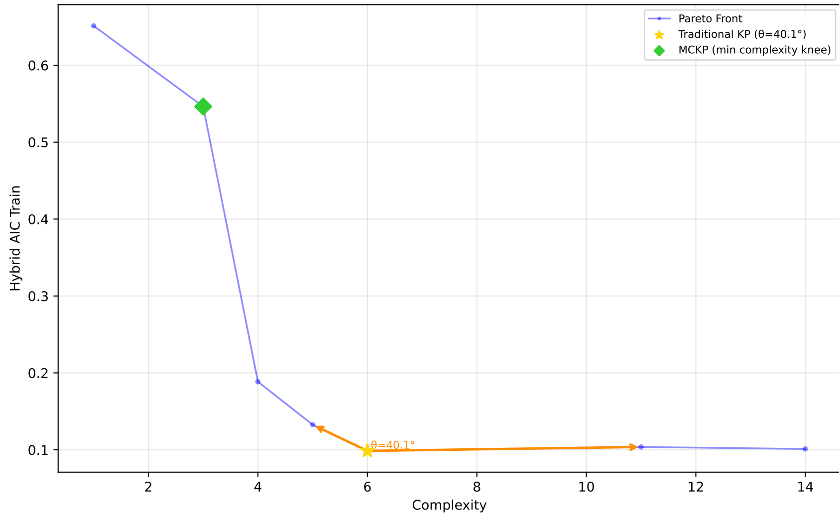
523_analcatdata_neavote - Run 7 - MVP - Hybrid AIC Train \lambda_1=0.00 , \lambda_2=0.40 , \lambda_3=0.00 | Difficulty: 1.00 | Method: hmr
