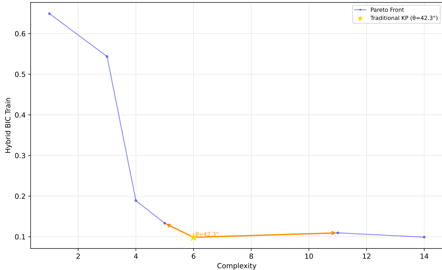
523_analcatdata_neavote - Run 7 - MVP - Hybrid BIC Train \lambda_1=0.00 , \lambda_2=0.10 , \lambda_3=0.00 | Difficulty: 1.00 | Method: hmr
