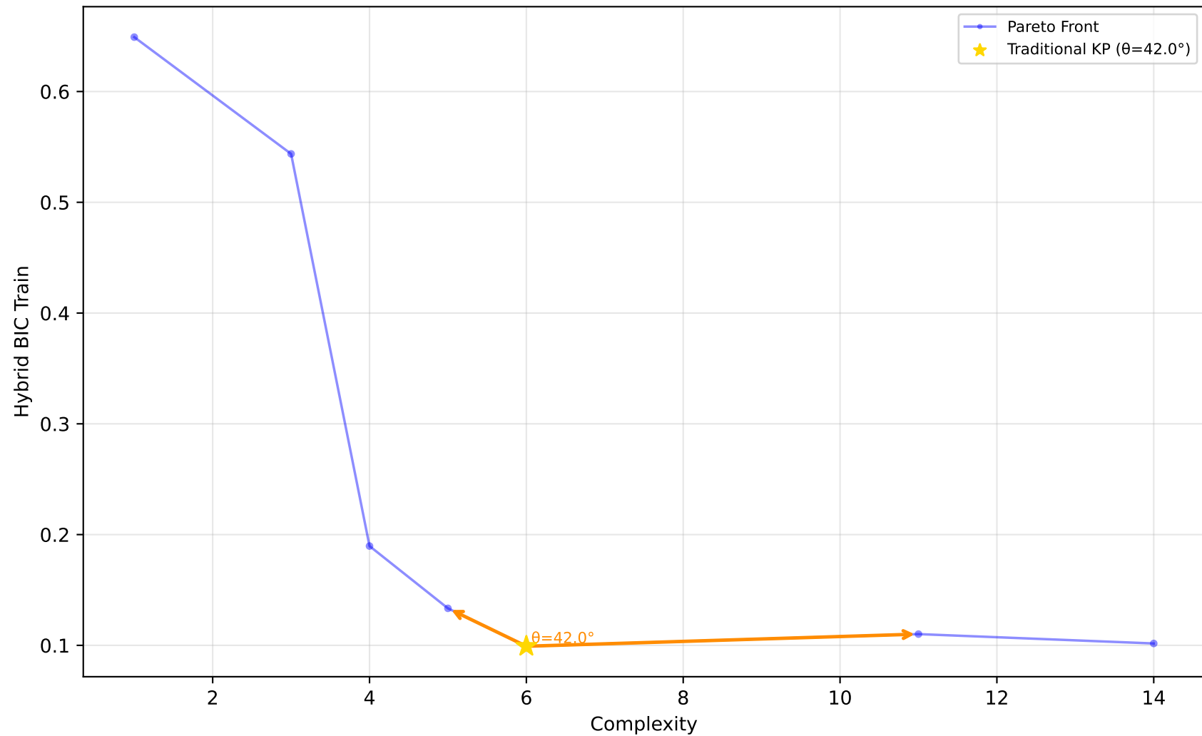
523_analcatdata_neavote - Run 7 - MVP - Hybrid BIC Train \lambda_1=0.00 , \lambda_2=0.40 , \lambda_3=0.00 | Difficulty: 1.00 | Method: hmr
