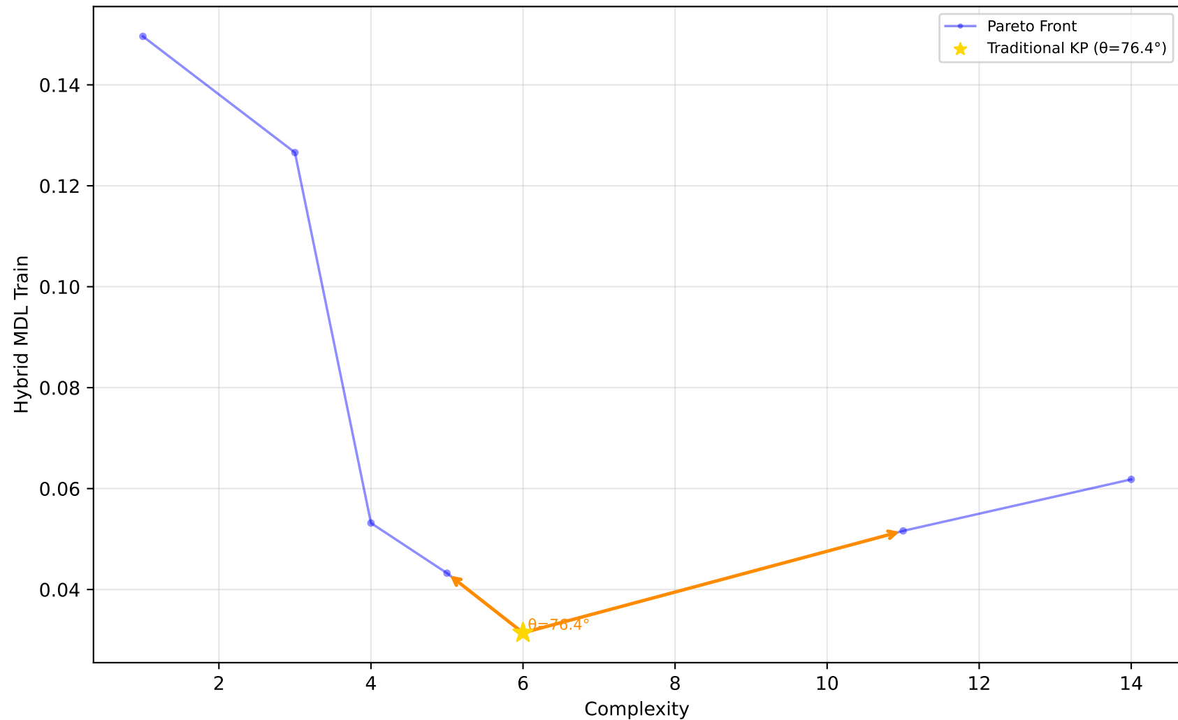
523_analcatdata_neavote - Run 7 - MVP - Hybrid MDL Train \lambda_1=0.00, \lambda_2=0.10, \lambda_3=0.00 | Difficulty: 1.00 | Method: hmr
