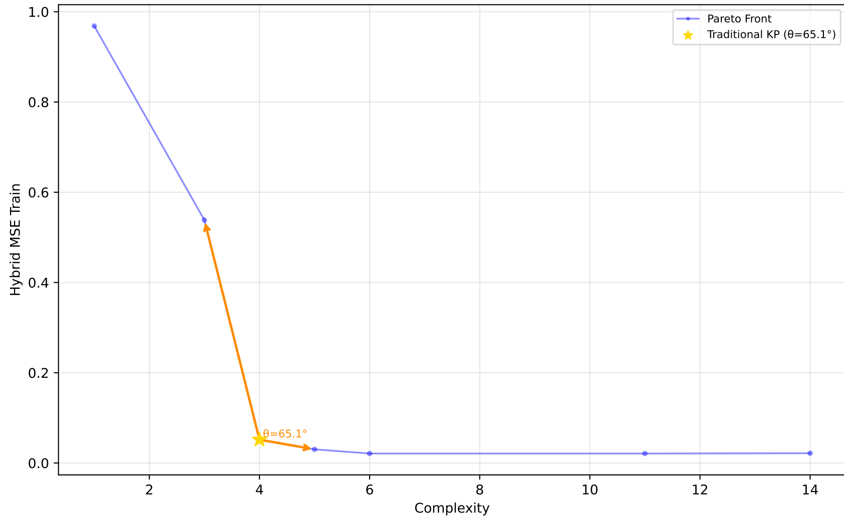
523_analcatdata_neavote - Run 7 - MVP - Hybrid MSE Train \lambda_1=0.00, \lambda_2=0.10, \lambda_3=0.00 | Difficulty: 1.00 | Method: hmr
