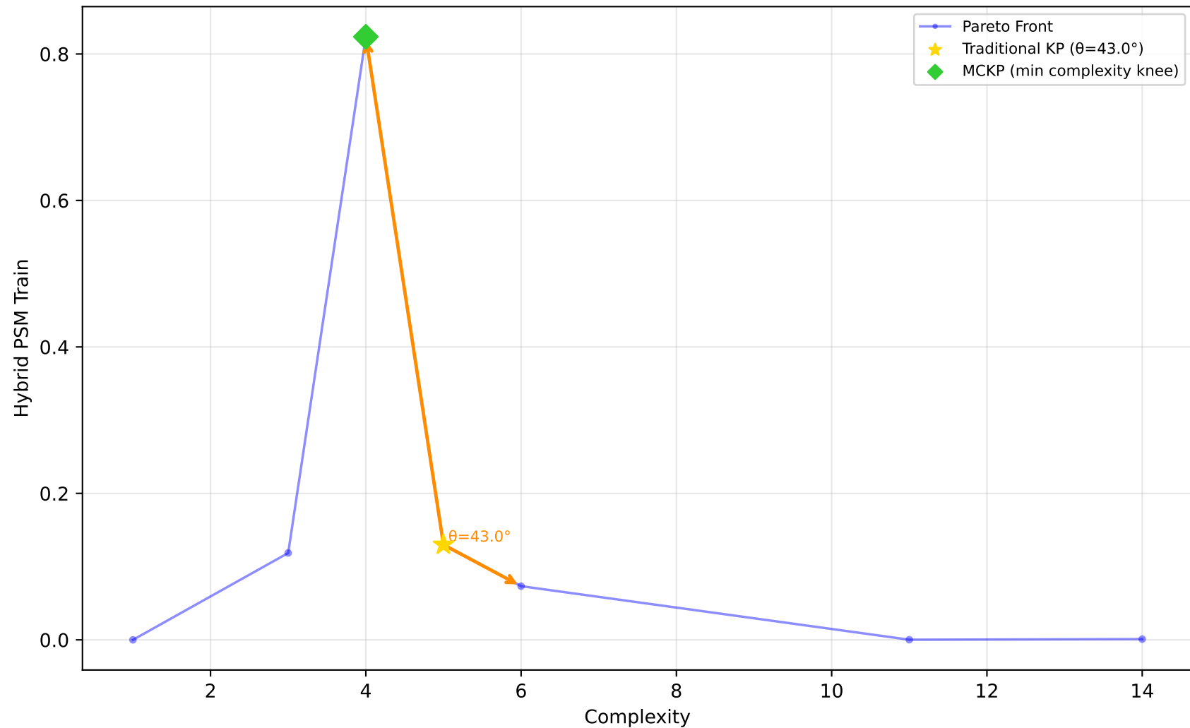
523_analcatdata_neavote - Run 7 - MVP - Hybrid PSM Train \lambda_1=0.00, \lambda_2=0.10, \lambda_3=0.00 | Difficulty: 1.00 | Method: hmr
