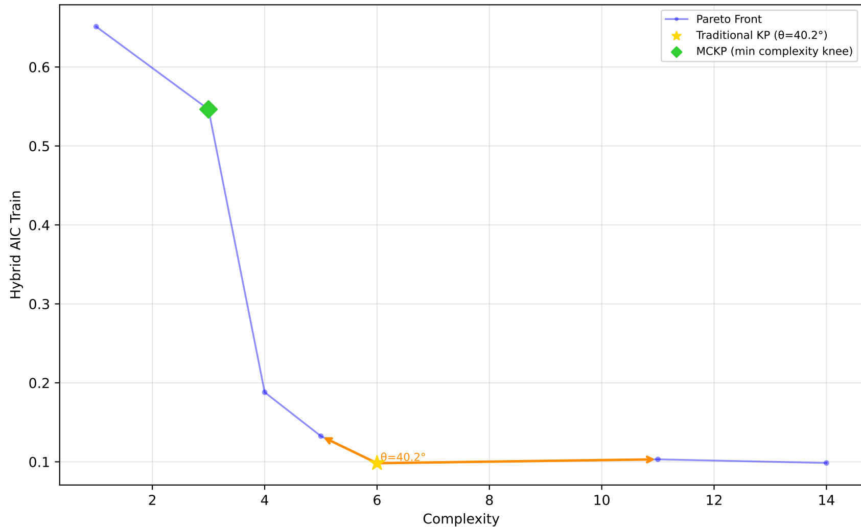
523_analcatdata_neavote - Run 7 - SVP - Hybrid AIC Train \lambda_1=0.00 , \lambda_2=0.20 , \lambda_3=0.00 | Difficulty: 1.00 | Method: hmr
