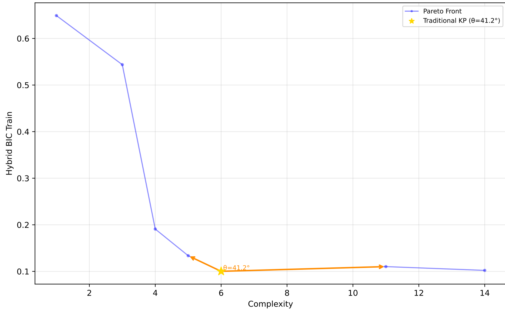
523_analcatdata_neavote - Run 7 - SVP - Hybrid BIC Train \lambda_1=0.00, \lambda_2=0.90, \lambda_3=0.00 | Difficulty: 1.00 | Method: hmr
